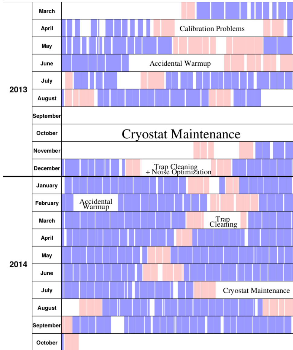
Figure 3.13: Timeline break down of the CUORE-0 data taking. The blue intervals represent physics data taking, red/pink intervals represent calibration data taking, and white represents detector down time.
