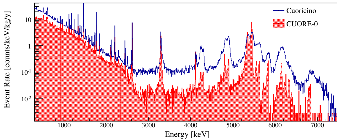
Figure 3.16: Spectrum of events with energy between 300 keV and 7500 keV measured in CUORICINO (blue/line) and CUORE-0 (red/solid).
