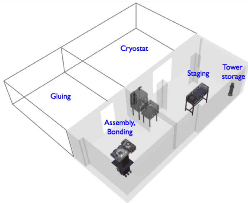
Figure 3.3: Sketch of the first floor (clean room) of the CUORE hut, with relevant tower assembly activities for each room labeled. Note: the entrance/dressing room is not shown in this figure.
