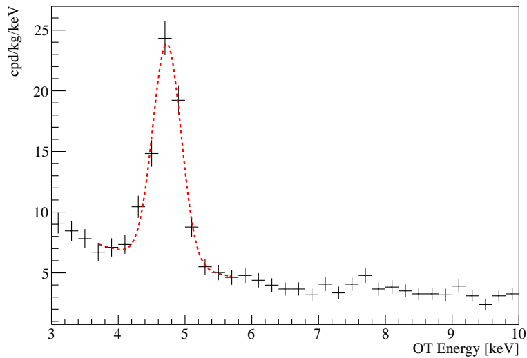
Figure 5.7: Result of the fit of the 4.7 keV peak in the CUORICINO spectrum.
