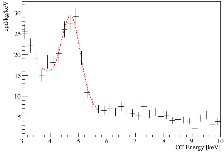
Figure 5.6: Result of the fit of the 4.7 keV peak in the CCVR2 spectrum.
